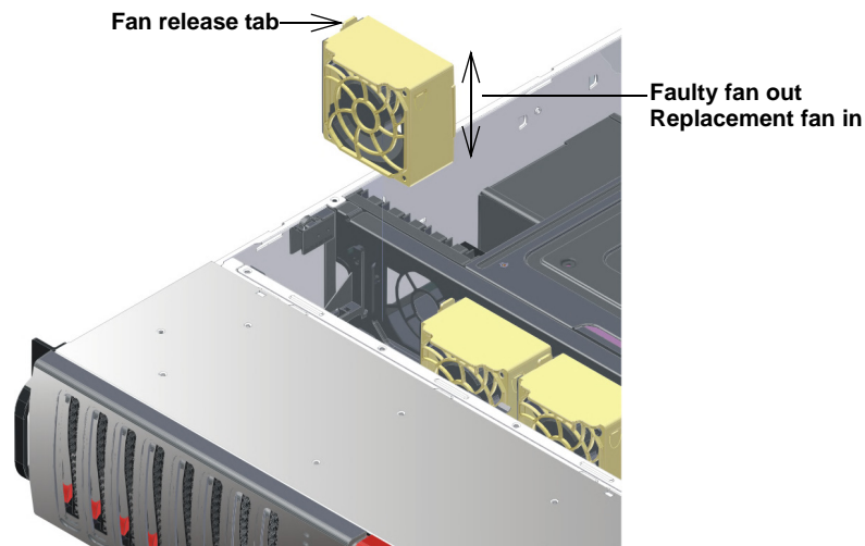
Figure 2 Replacing a DSS200 Front System Fan
