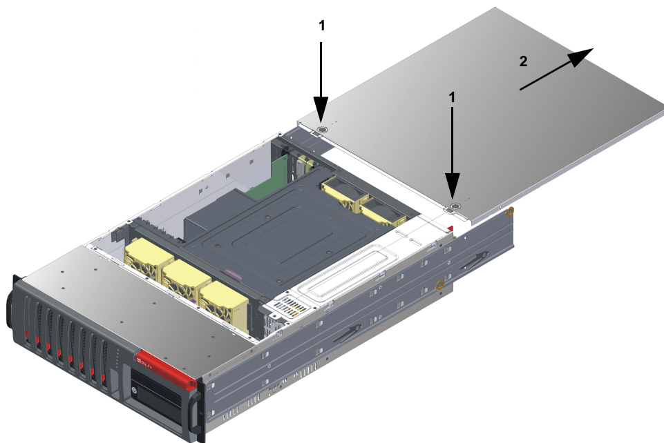
Figure 1 Removing the DSS200 Chassis Cover
