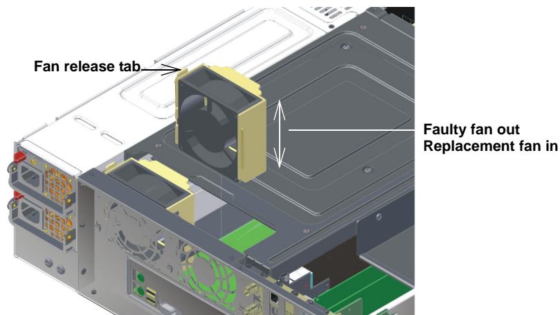
Figure 3 Replacing a DSS200 Rear System Fan
