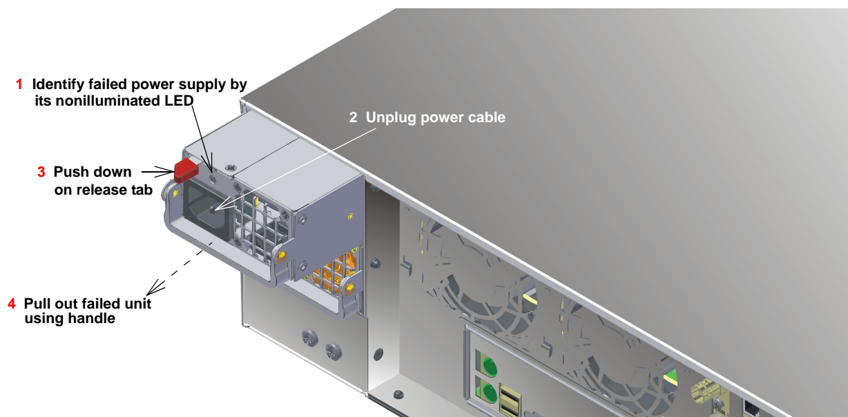
Figure 2 Removing the Failed DSS200 Power Supply
